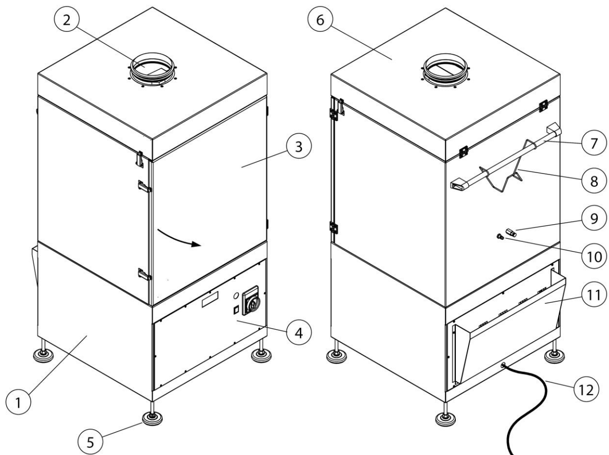
Fig. 1: Functional description
