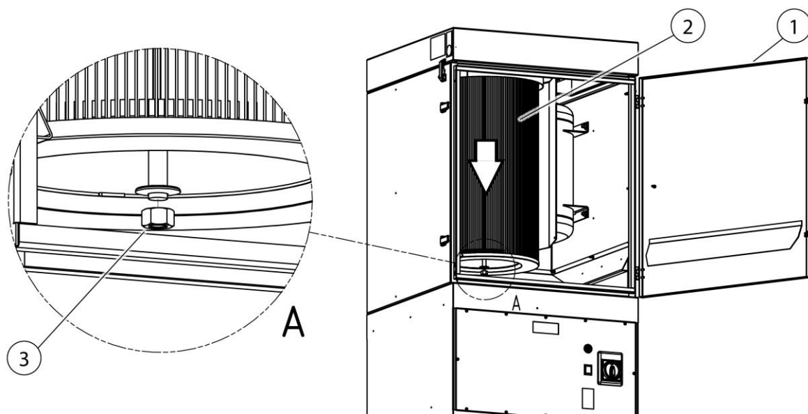
Fig. 9: Changing filters
